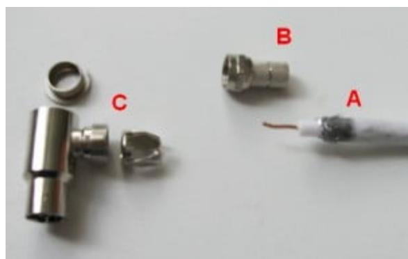
A: coax-kabel. B: F-connector. C: Coax-antennestik i metal.
